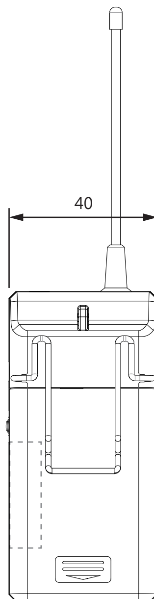
Rear view
