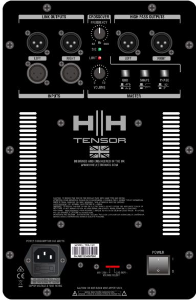
CONTROL PANEL
